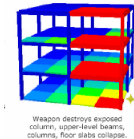
Figure 19 – BlastFX Modeling (NorthrupGrumman)
